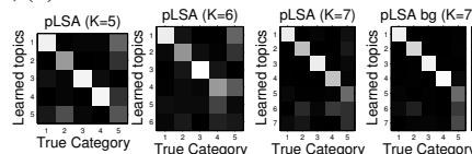
Figure 4: Confusion tables for Expt. (2) for increasing number of topics ( K=5,6,7 ) and with 7 topics and fixed background respectively. Brightness indicates number. The ideal is bright down the diagonal. Note how the background (category 5) splits into 2 and 3 topics (for K=6 and 7 respectively) and that some amount of the confusion between categories and background is removed.
