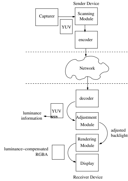
Fig. 4. Architecture and major components of our online greedy display power saving system.
