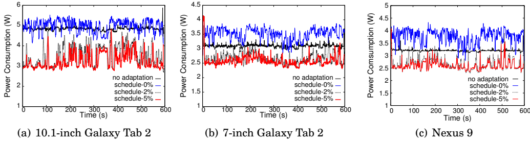
Fig. 7. Measured results: power consumed by the entire device with backlight scaling.
