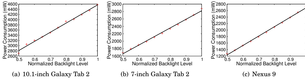
Fig. 6. Display power consumption model.
