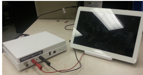
Fig. 5. Power measurement setup.
