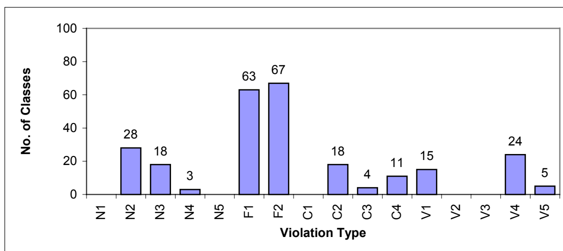
Figure 1. Violation type vs. number of classes
