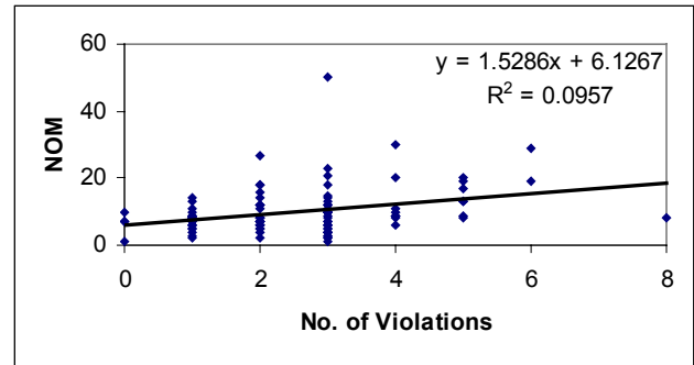
Figure 4. Scatter plot of number of violations vs. NOM
