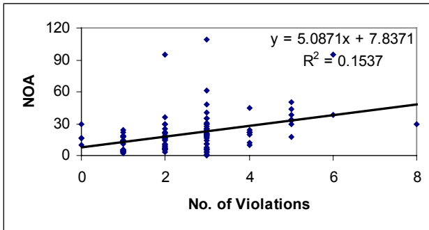
Figure 5. Scatter plot of number of violations vs. NOA
