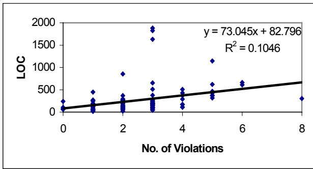
Figure 3. Scatter plot of number of violations vs. LOC
