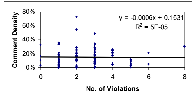
Figure 6. Scatter plot of number of violations vs. comment density
