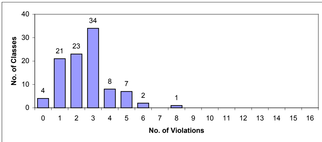
Figure 2. Number of violations vs. number of classes
