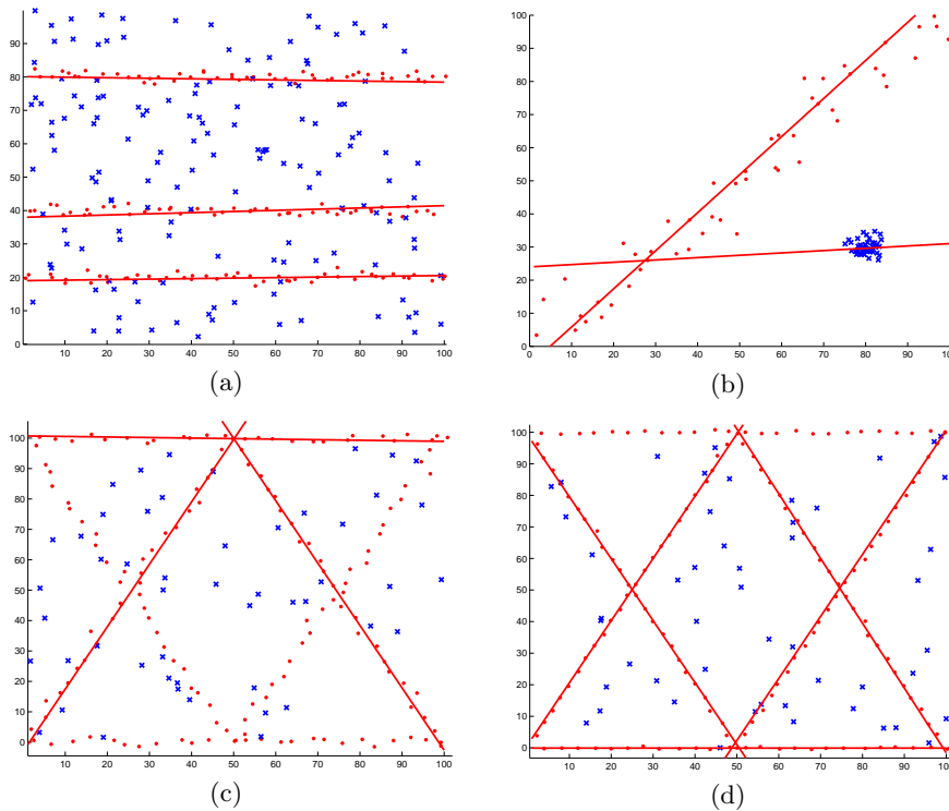
Fig. 6. The line fitting experiments, inliers are denoted as red '.', outliers are denoted as blue 'x'.
