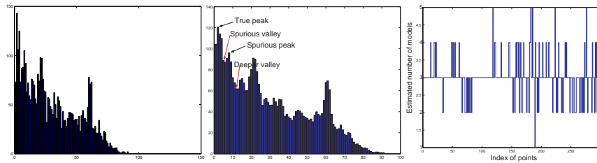
Fig. 2. Residual histogram Fig. 3. Peak identification Fig. 4. Estimated number of a point. for the histogram. numbers of models.
