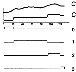
Figure 51.20. A visualization of the APCA dimensionality reduction technique
