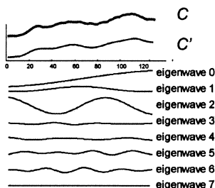
Figure 51.17. A visualization of the SVD dimensionality reduction technique.
