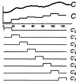
Figure 51.19. A visualization of the PAA dimensionality reduction technique
