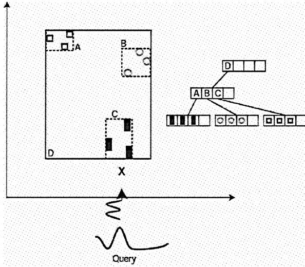
Figure 51.6. Hierarchical organization using an R-tree
