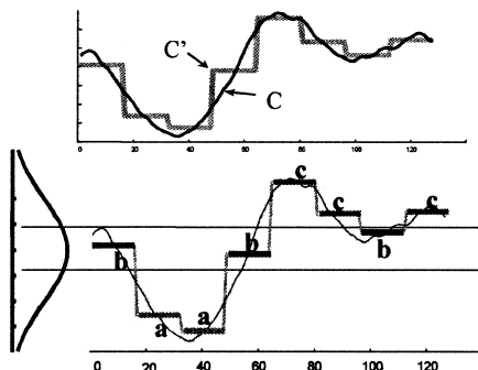
Figure 51.21. A visualization of the SAX dimensionality reduction technique
