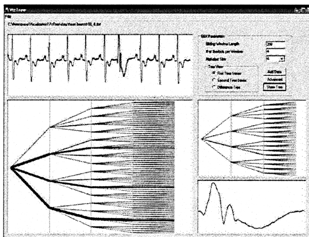
Figure 51.11. ECG data with anomaly is shown. While the subsequence tree can be used to identify motifs, it can be used for simple anomaly detection as well
