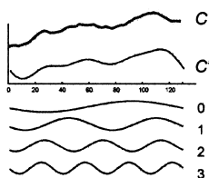
Figure 51.15. A visualization of the DFT dimensionality reduction technique
