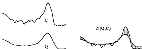
Figure 51.1. The intuition behind the Euclidean distance metric
