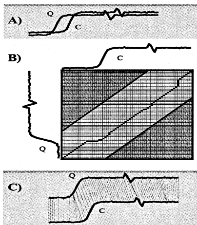
Figure 51.4. A) Two similar sequences Q and C, but out of phase. B) To align the sequences, we construct a warping matrix, and search for the optimal warping path, shown with solid squares. Note that the “corners” of the matrix (shown in dark gray) are excluded from the search path (specified by a warping window of size w ) as part of an Adjustment Window condition. C) The resulting alignment
