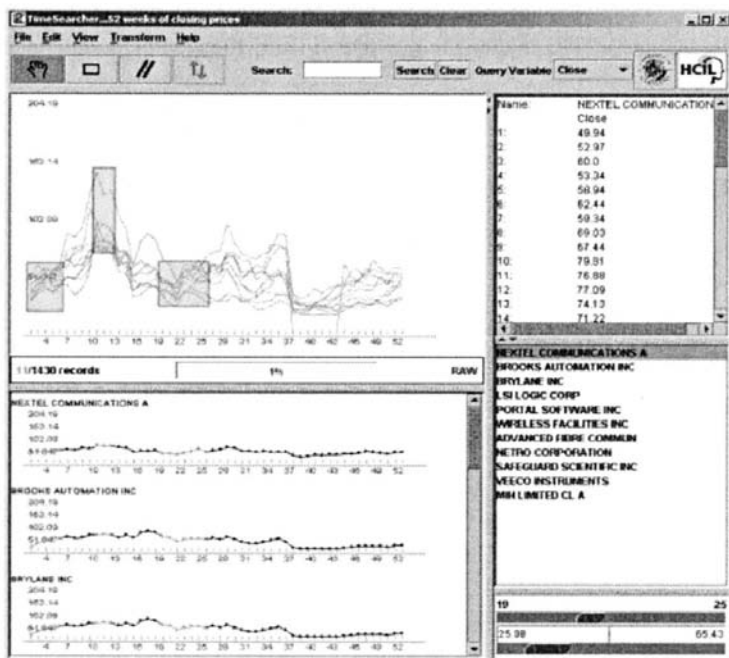
Figure 51.8. The TimeSearcher visual query interface. A user can filter away sequences that are not interesting by insisting that all sequences have at least one data point within the query boxes
