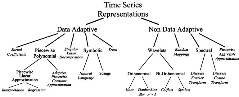
Figure 51.14. A hierarchy of time series representations
