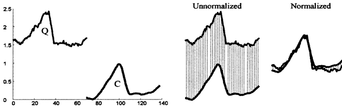
Figure 51.2. A visual intuition of the necessity to normalize time series before measuring the distance between them. The two sequences Q and C appear to have approximately the same shape, but have different offsets in Y-axis. The unnormalized data greatly overstate the subjective dissimilarity distance. Normalizing the data reveals the true similarity of the two time series.
