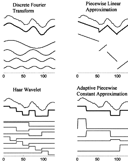
Figure 51.22. Four popular representations of time series. For each graphic, we see a raw time series of length 128. Below it, we see an approximation using 1/8 of the original space. In each case, the representation can be seen as a linear combination of basis functions. For example, the Discrete Fourier representation can be seen as a linear combination of the four sine/cosine waves shown in the bottom of the graphics.
