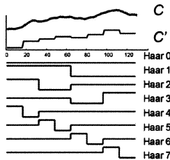
Figure 51.16. A visualization of the DWT dimensionality reduction technique
