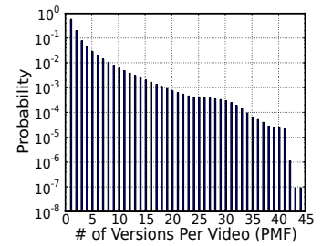
Fig. 4. # of Versions Per Video (PMF)
