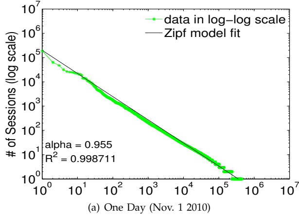
Fig. 9. Video Popularity Distribution
