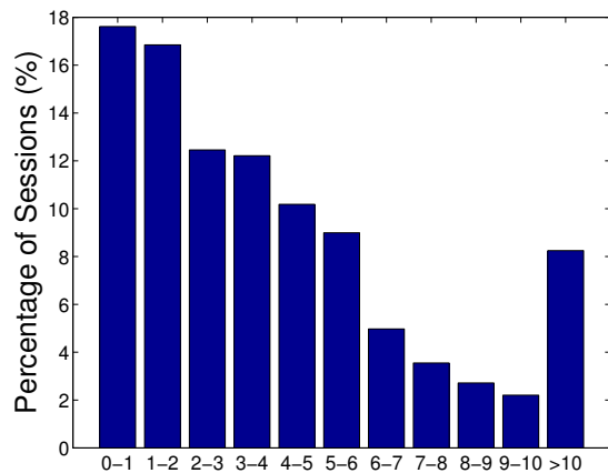
Fig. 10. % of Sessions for Videos of Different Length (minute)
