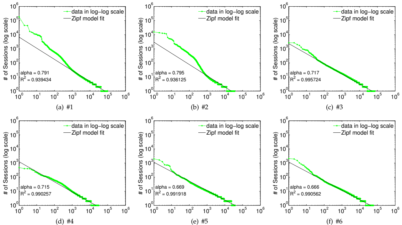
Fig. 11. Daily Video Popularity Distribution per ISP
