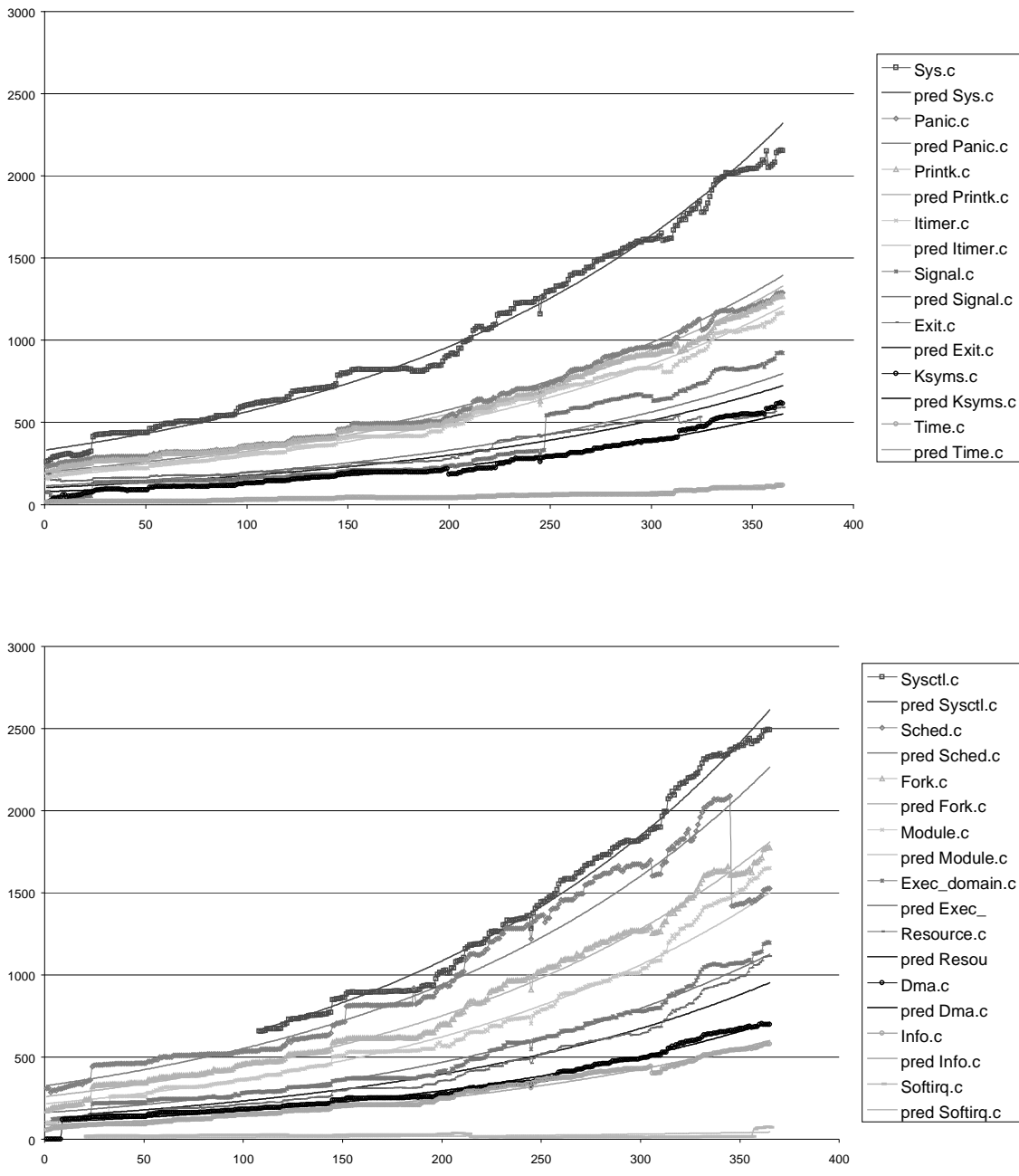
Figure 1. Graphs of measured and predicted common coupling versus version number. The measured common coupling is represented by discrete points, the predicted common coupling by a line.
